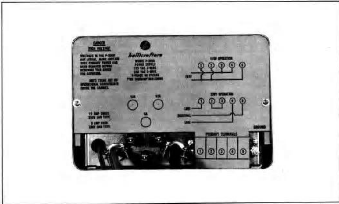
Figure 4. Model P-2000 Power Supply, Rear View.
