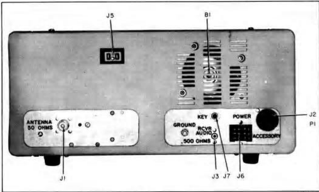
Figure 3. Model SR-2000 Transceiver, Rear View.
