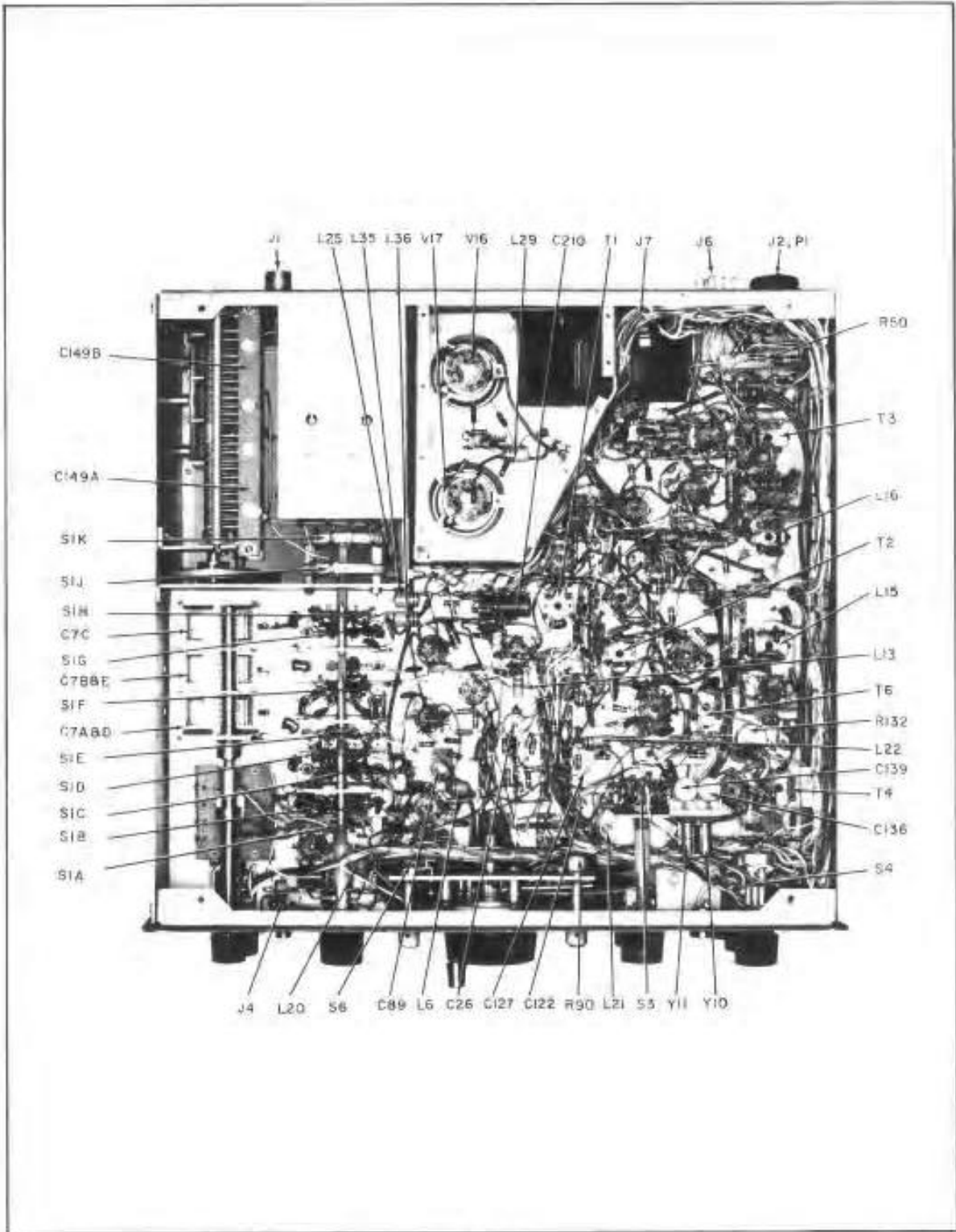
Figure 14. Model SR-2000 Bottom View, Component Location.
