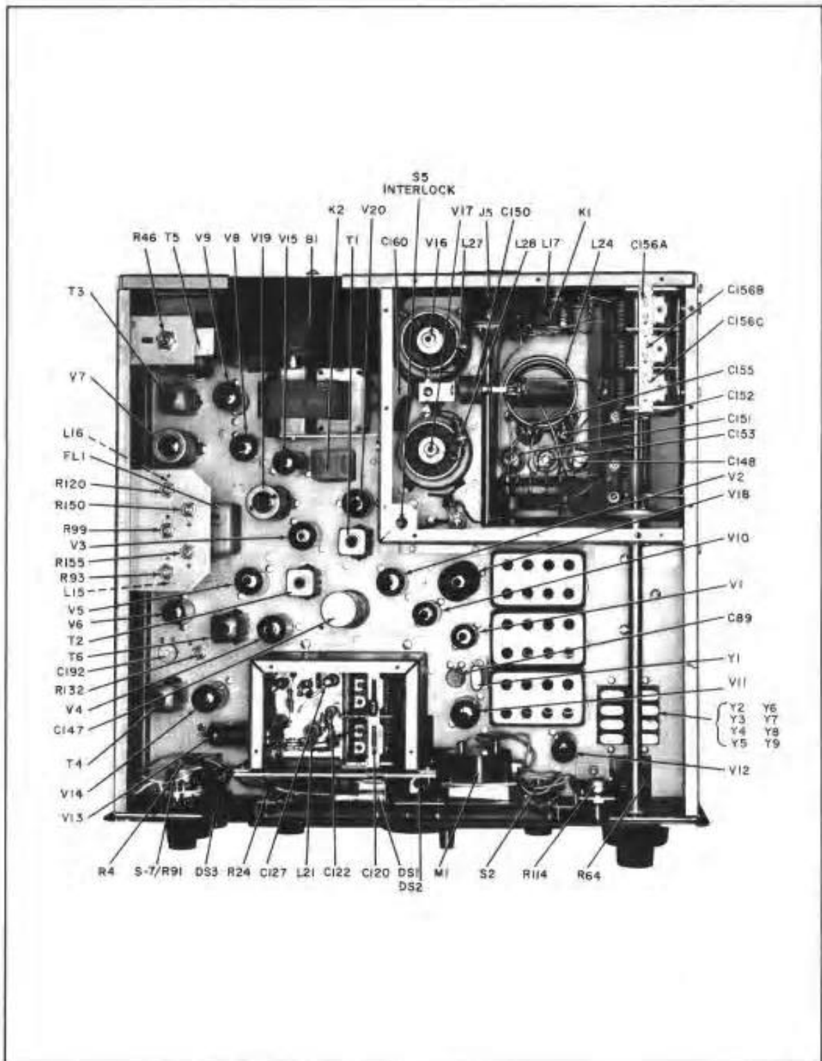
Figure 13. Model SR-2000 Top View, Component Location.
