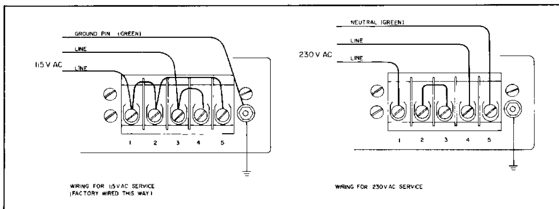
Figure 2. Model P-2000 Power Supply, Primary Power Connections.
