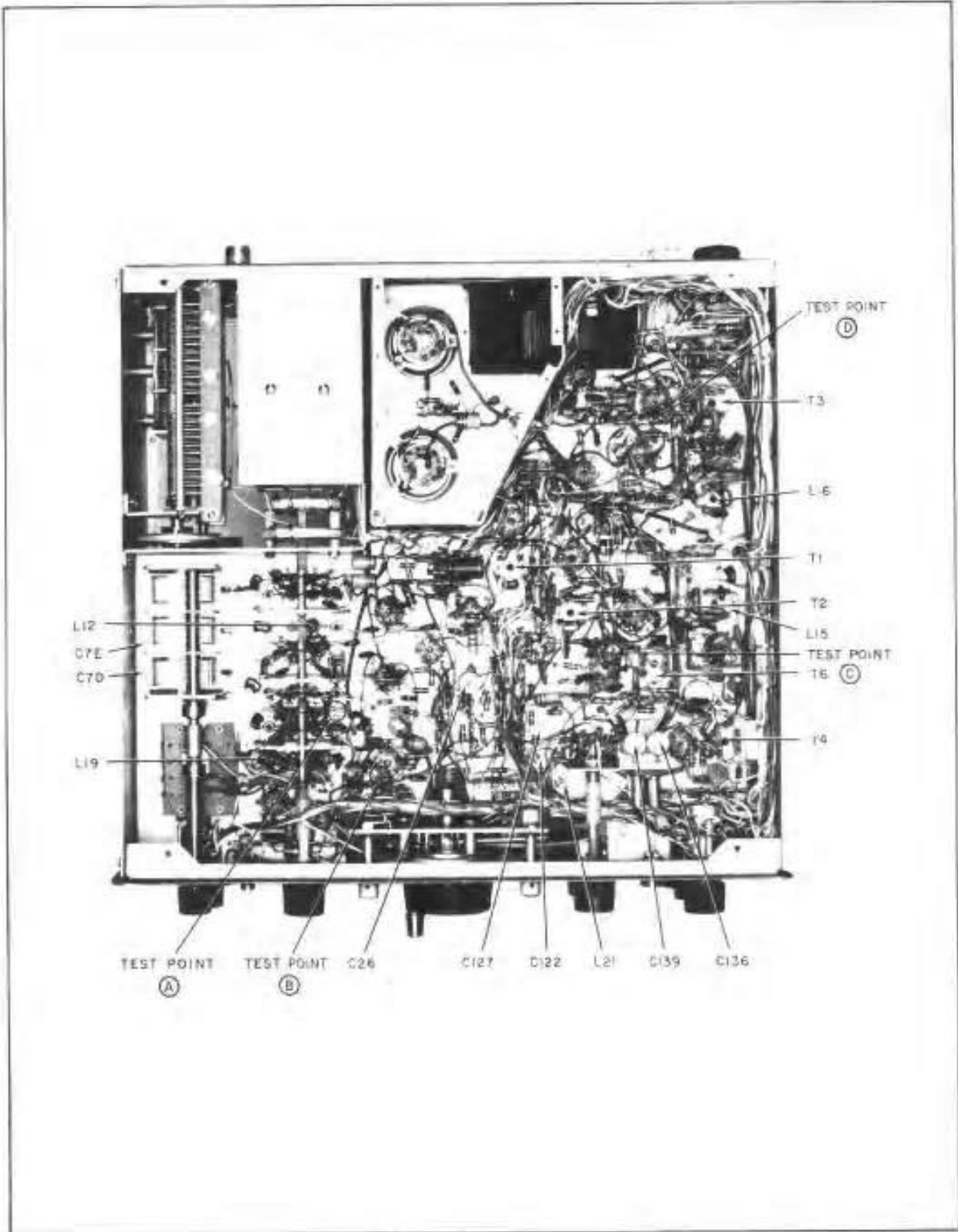
Figure 16. Model SR-2000 Bottom View, Alignment Adjustments.
